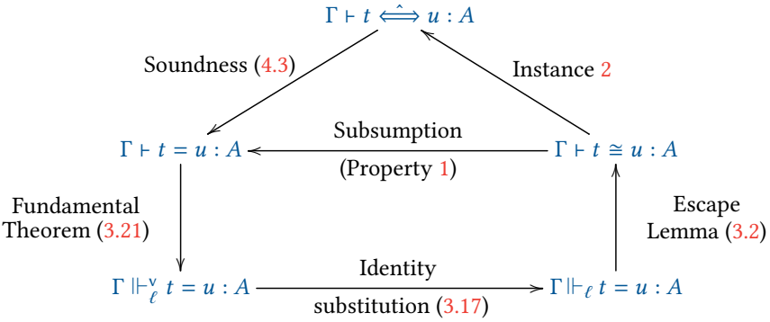
Fig. 5. Proof outline.
