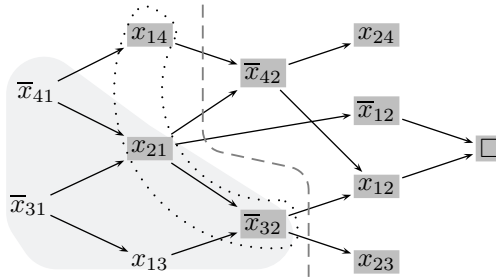
Figure 2.2: The conflict graph G for OP_4 with a proper sub conflict graph and the corresponding cut. The conflict clause of the subgraph is \mathcal{C} = (\bar{x}_{14} \vee \bar{x}_{21} \vee x_{32}) . It is possible to include G and the UP-graph G|_{\bar{x}_{32}} in a compatible set of subgraphs and to learn the clauses \mathcal{C} and \{\bar{x}_{32}, x_{41}, x_{31}\} .
