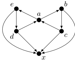
Fig. 3. Output gadget. All players have payoffs as in Figure 2. Player x must play action 0 in every pure equilibrium of the game.
