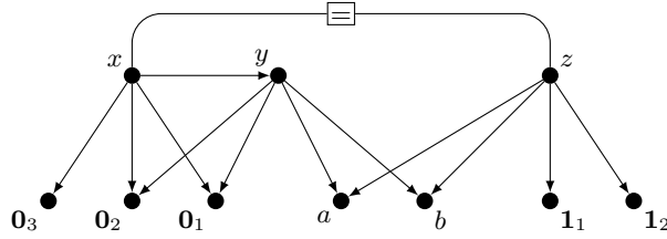
Fig. 7. NOR gadget. Payoffs are identical to those in Figure 6. A construction analogous to the one shown in Figure 4 is used to ensure that players x and z play the same action in every pure equilibrium.
