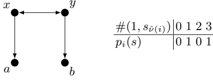
Fig. 4. Equality gadget. A pure equilibrium exists if and only if players a and b play the same action.
