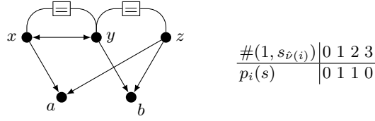
Fig. 5. NAND gadget. The construction of Figure 4 is used to ensure that players connected by “=” play the same action in every pure equilibrium.
