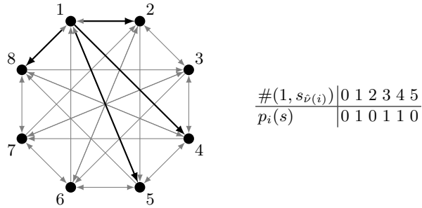
Fig. 6. Neighborhood graph and payoffs of a graphical game with eight players and neighborhoods of size four used in the proof of Theorem 5. The neighborhood graph satisfies rotational symmetry, the neighborhood of player 1 is highlighted.
